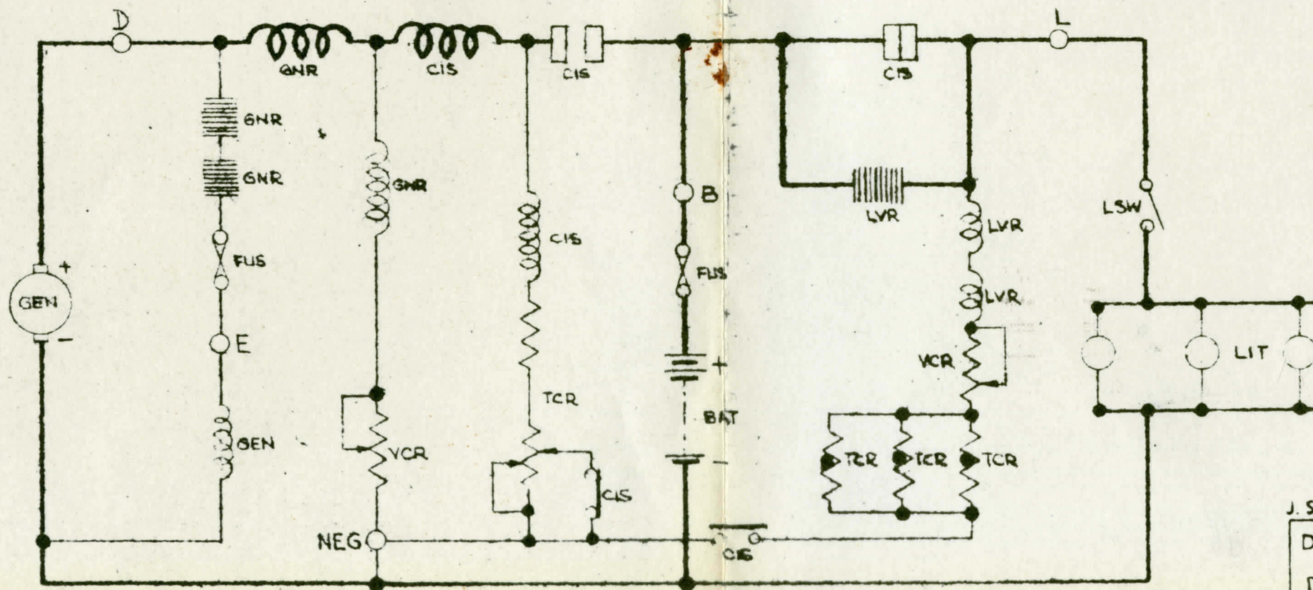
SCHEMATIC DIAGRAM
