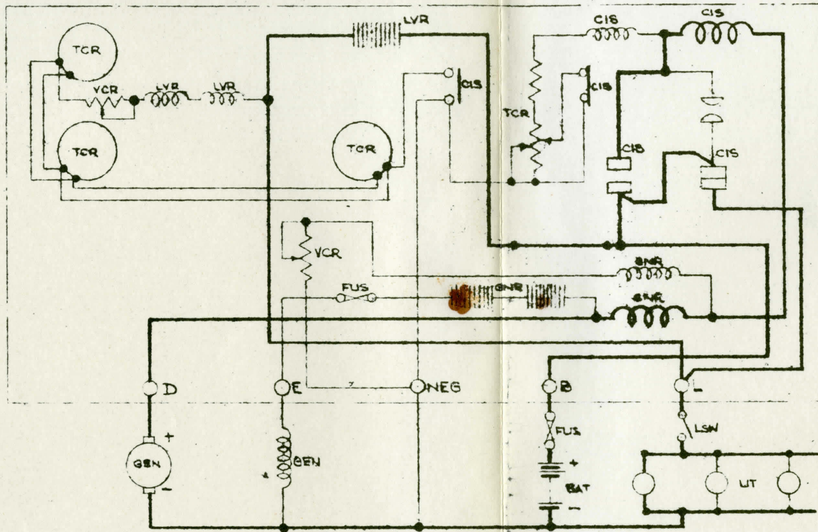
WIRING DIAGRAM
